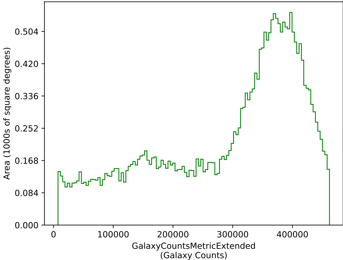
too_ignore_100_4v3.4_10yrs g: GalaxyCountsMetricExtended
