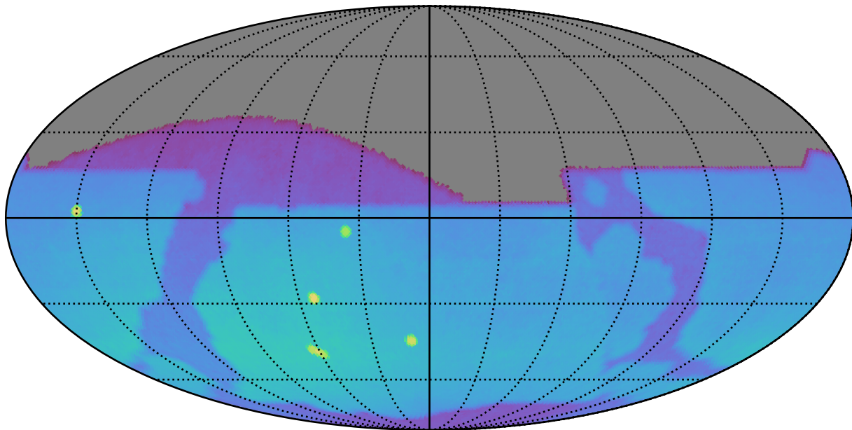
too_ignore_100_4v3.4_10yrs : Brown Dwarf, L4
