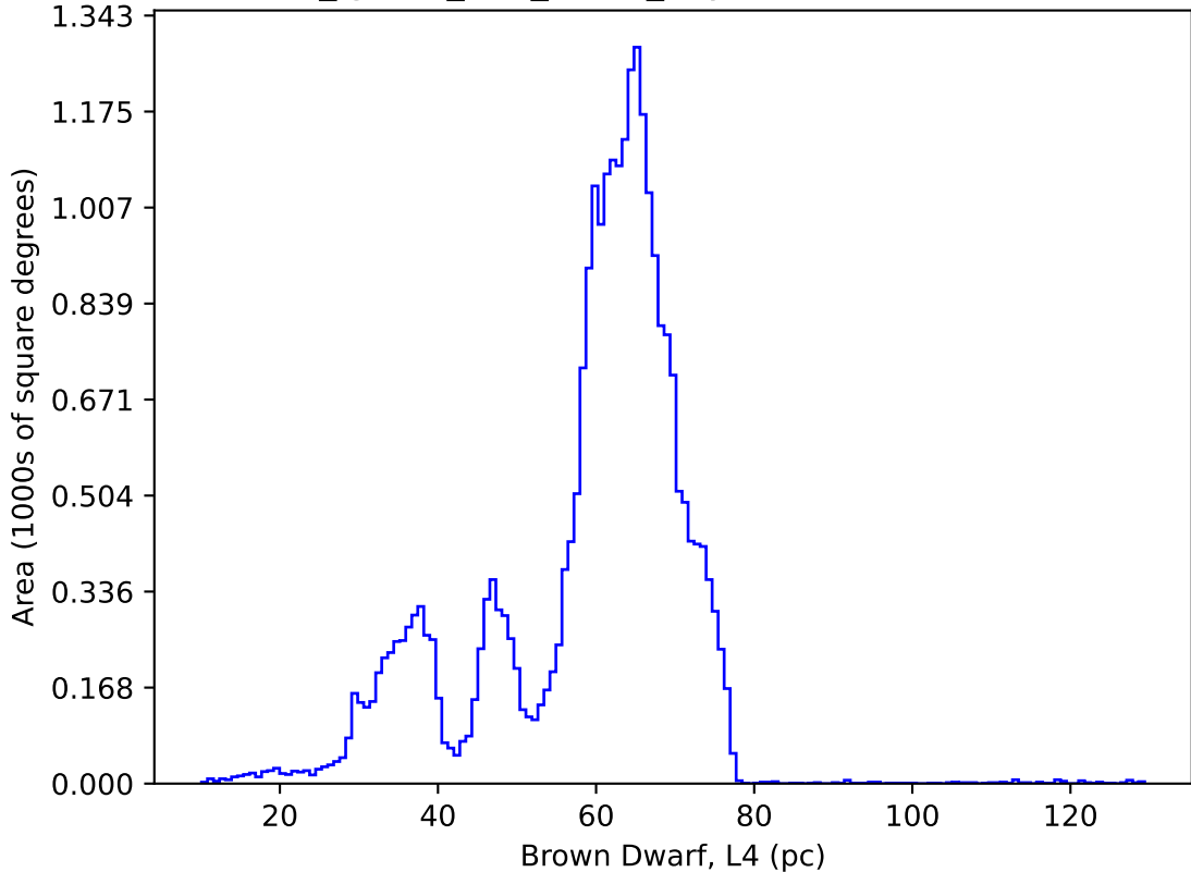
too_ignore_100_4v3.4_10yrs : Brown Dwarf, L4
