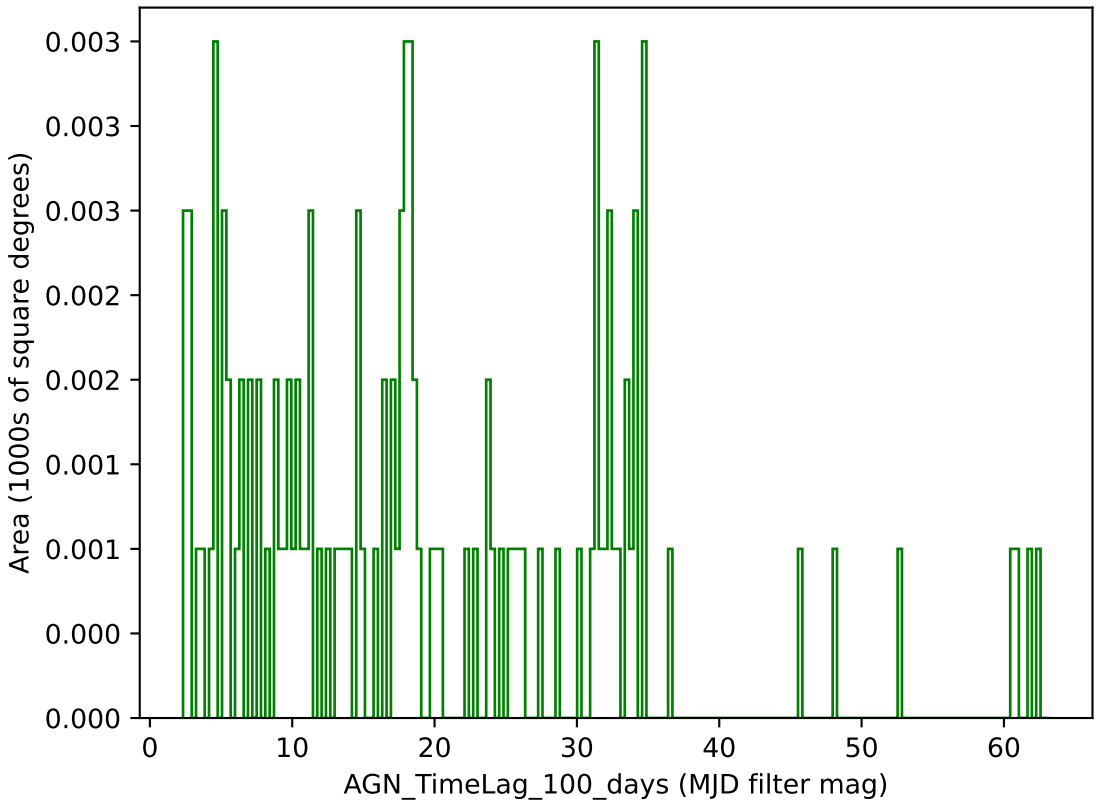
too_ignore_100_4v3.4_10yrs g band: AGN_TimeLag_100_days
