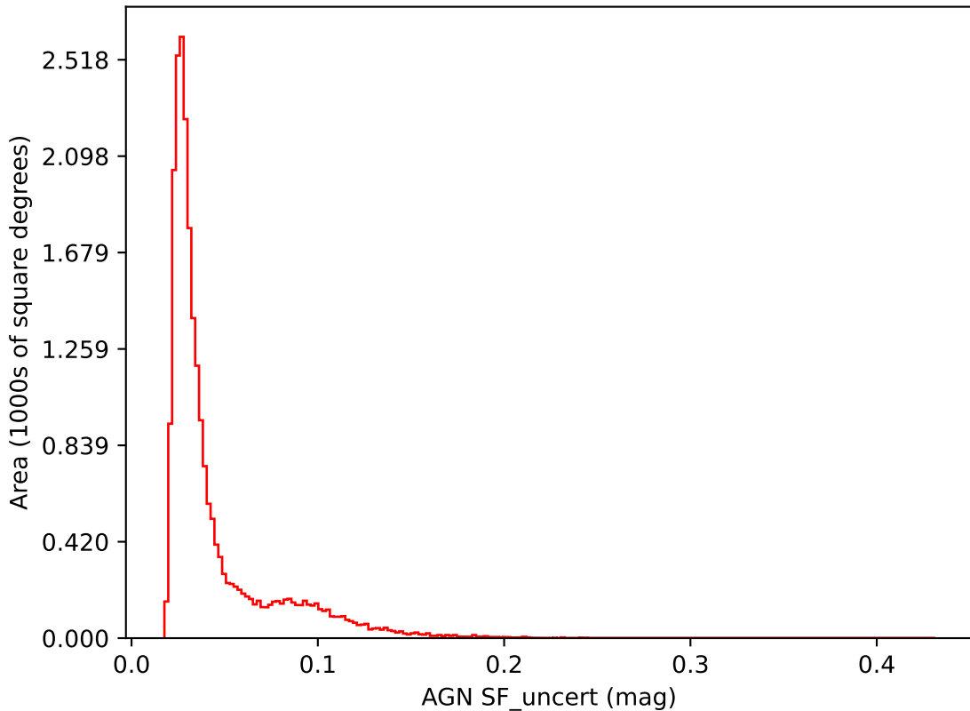
too_ignore_100_4v3.4_10yrs i band: AGN SF_uncert
