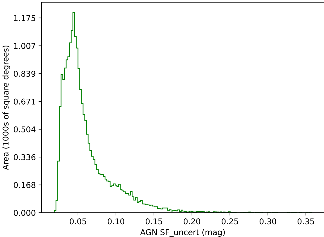
too_ignore_100_4v3.4_10yrs g band: AGN SF_uncert
