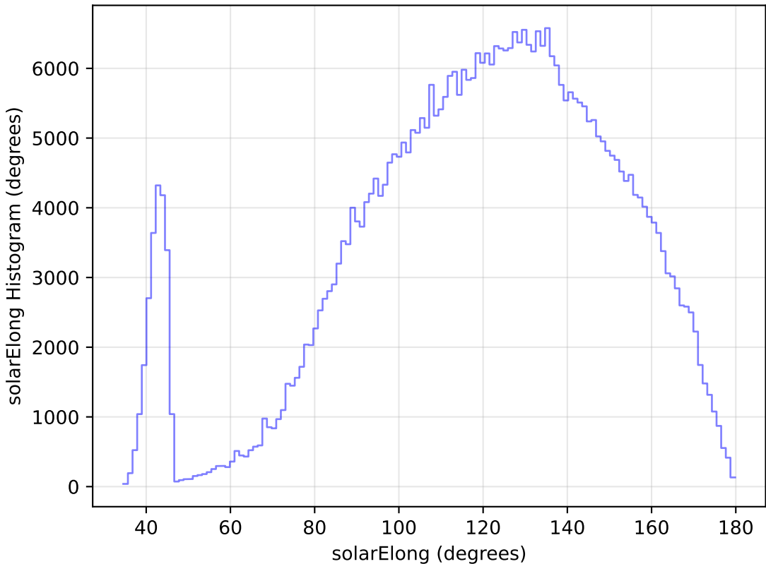
too_ignore_100_4v3.4_10yrs WFD z band: solarElong Histogram
