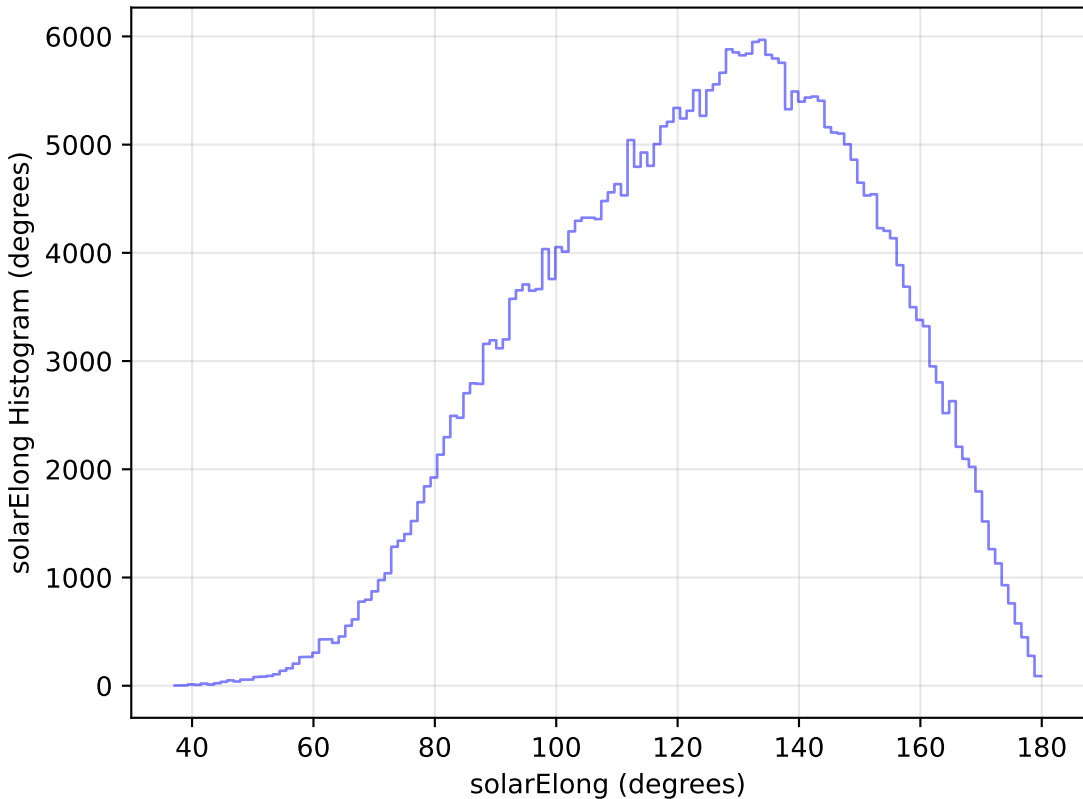
too_ignore_100_4v3.4_10yrs WFD y band: solarElong Histogram
