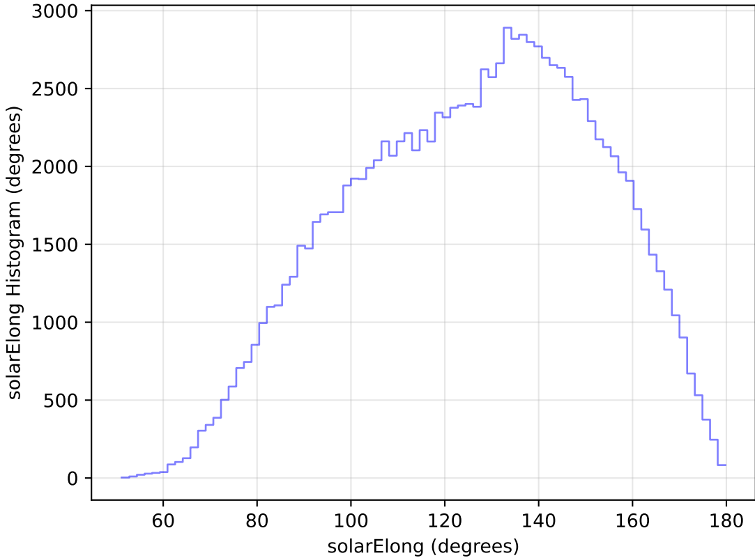
too_ignore_100_4v3.4_10yrs WFD u band: solarElong Histogram
