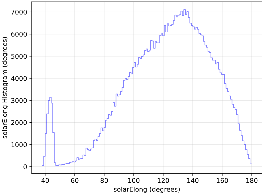
too_ignore_100_4v3.4_10yrs WFD r band: solarElong Histogram
