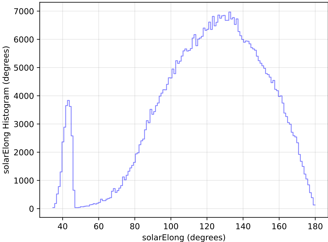
too_ignore_100_4v3.4_10yrs WFD i band: solarElong Histogram
