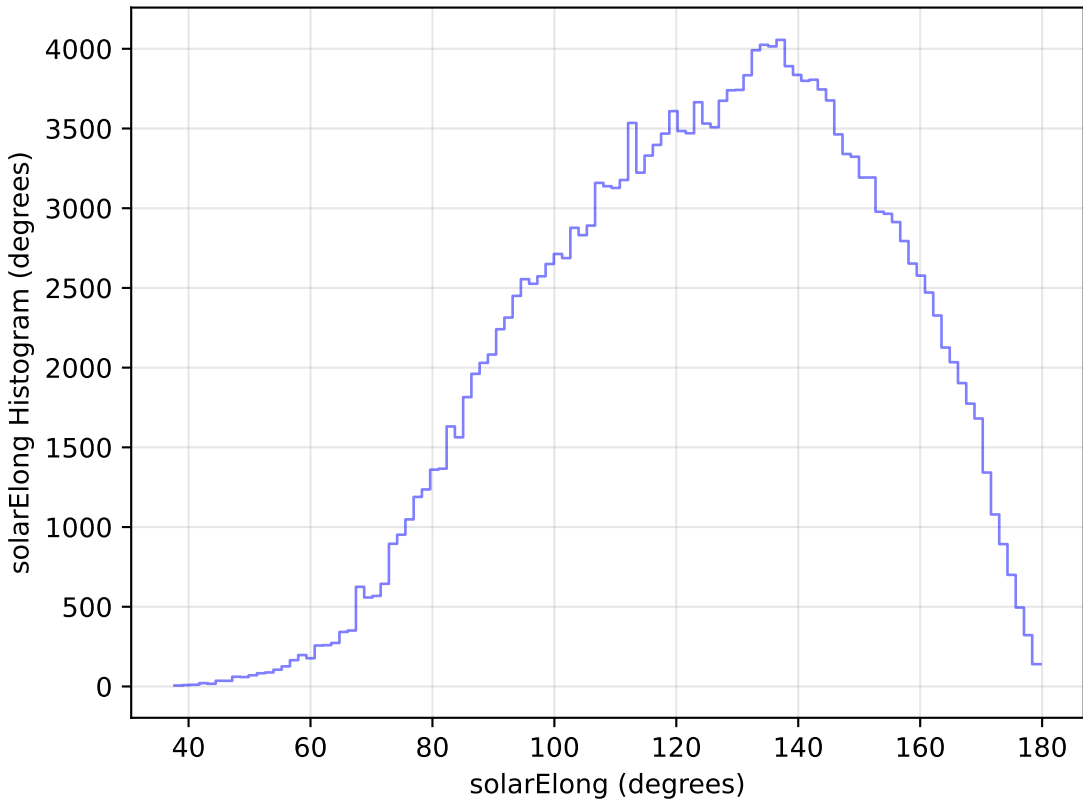
too_ignore_100_4v3.4_10yrs WFD g band: solarElong Histogram
