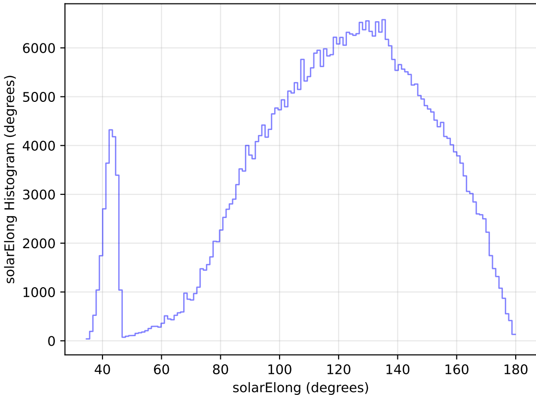
too_ignore_100_4v3.4_10yrs All sky z band: solarElong Histogram
