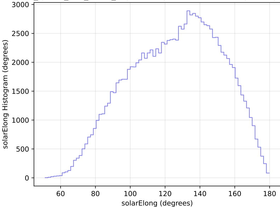
too_ignore_100_4v3.4_10yrs All sky u band: solarElong Histogram
