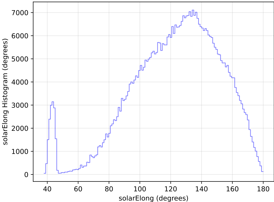
too_ignore_100_4v3.4_10yrs All sky r band: solarElong Histogram
