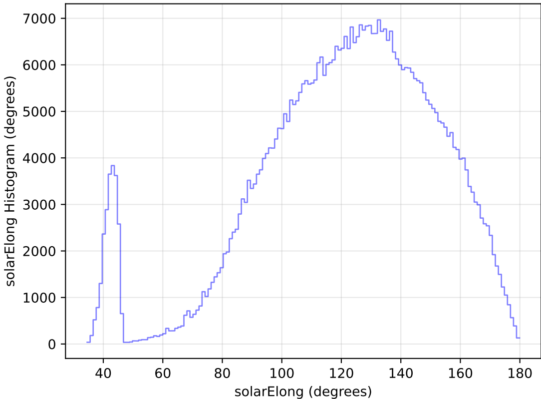
too_ignore_100_4v3.4_10yrs All sky i band: solarElong Histogram
