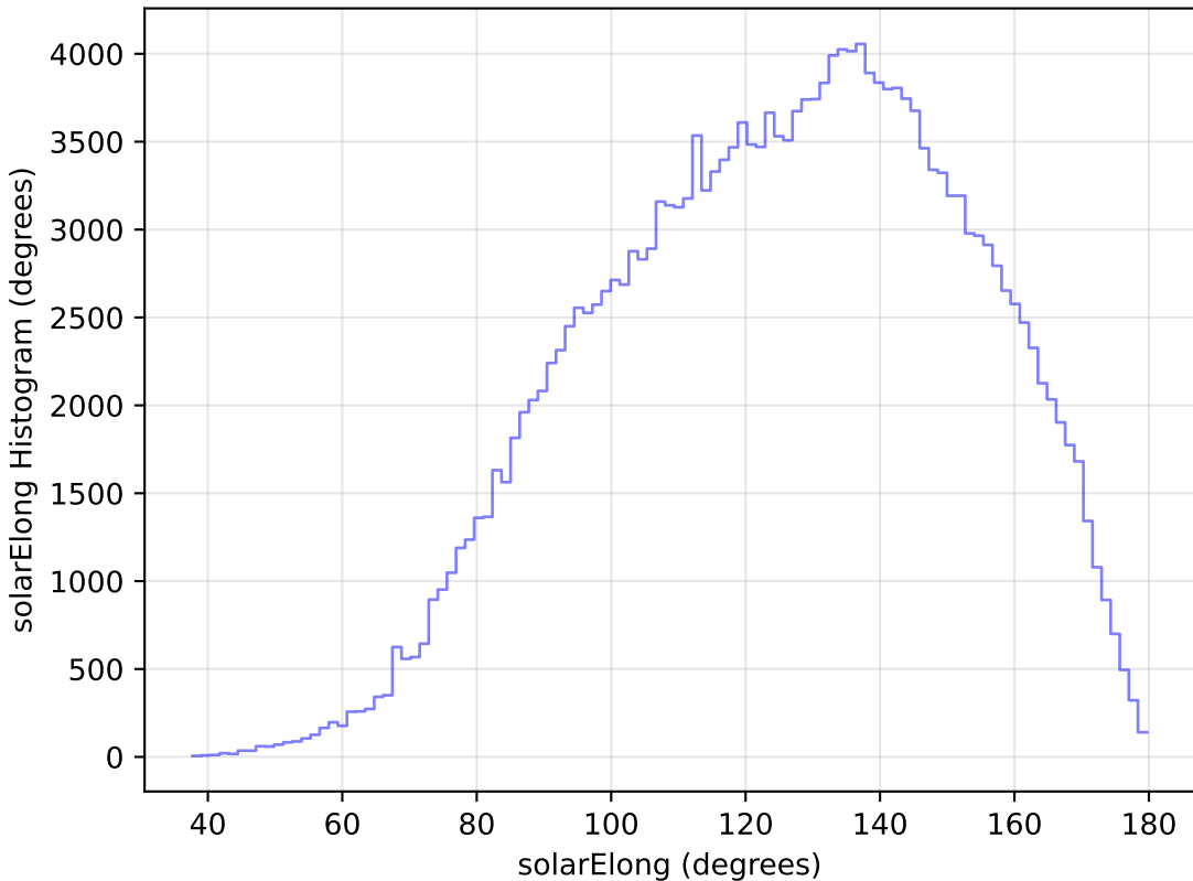
too_ignore_100_4v3.4_10yrs All sky g band: solarElong Histogram
