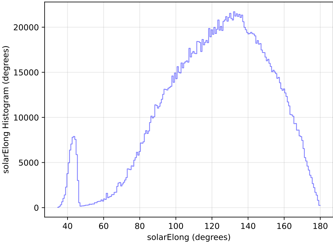
too_ignore_100_4v3.4_10yrs All sky all bands: solarElong Histogram
