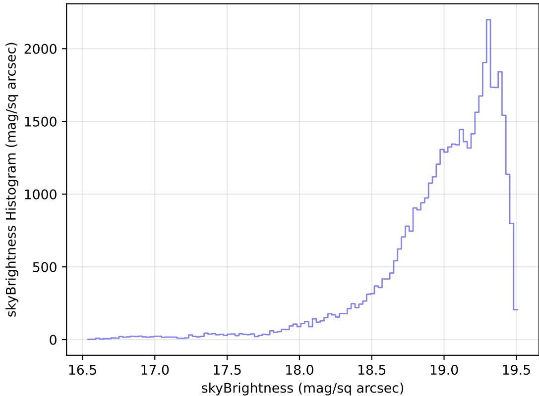
too_ignore_100_4v3.4_10yrs Yr 1 z band: skyBrightness Histogram
