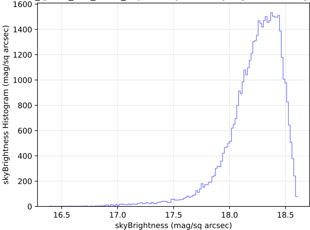
too_ignore_100_4v3.4_10yrs Yr 1 y band: skyBrightness Histogram
