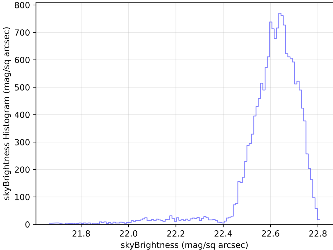
too_ignore_100_4v3.4_10yrs Yr 1 u band: skyBrightness Histogram
