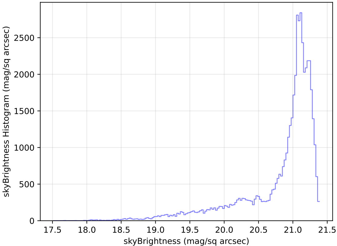
too_ignore_100_4v3.4_10yrs Yr 1 r band: skyBrightness Histogram
