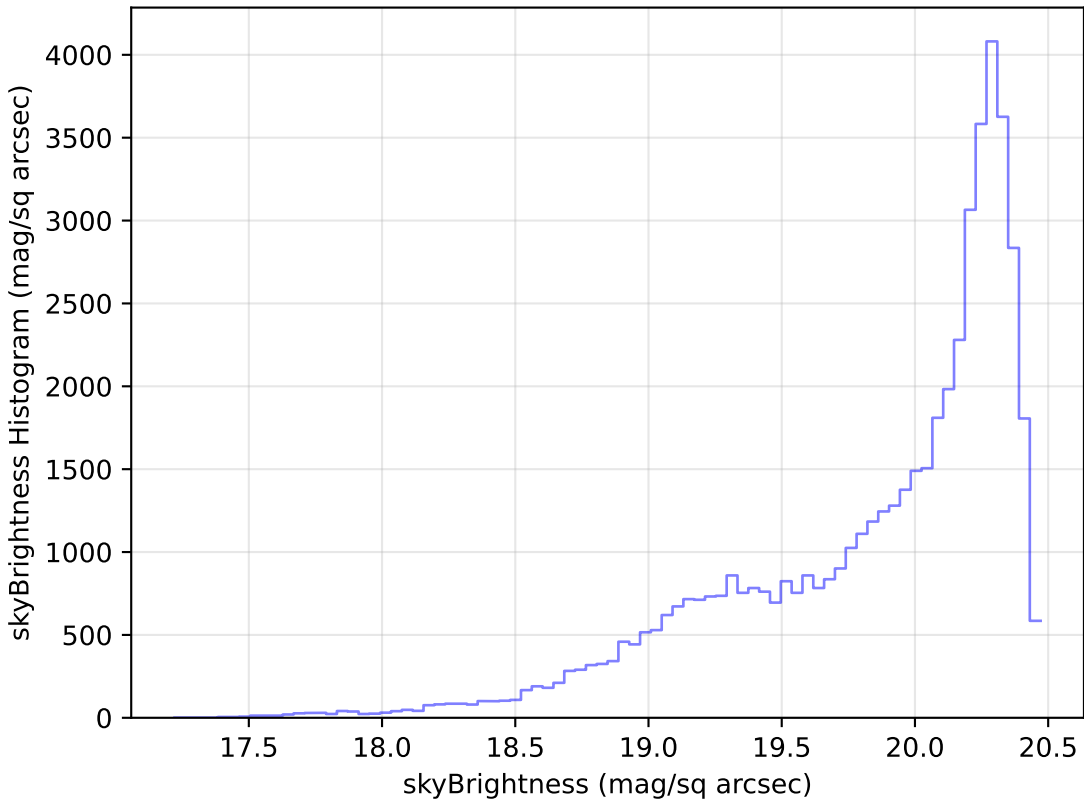
too_ignore_100_4v3.4_10yrs Yr 1 i band: skyBrightness Histogram
