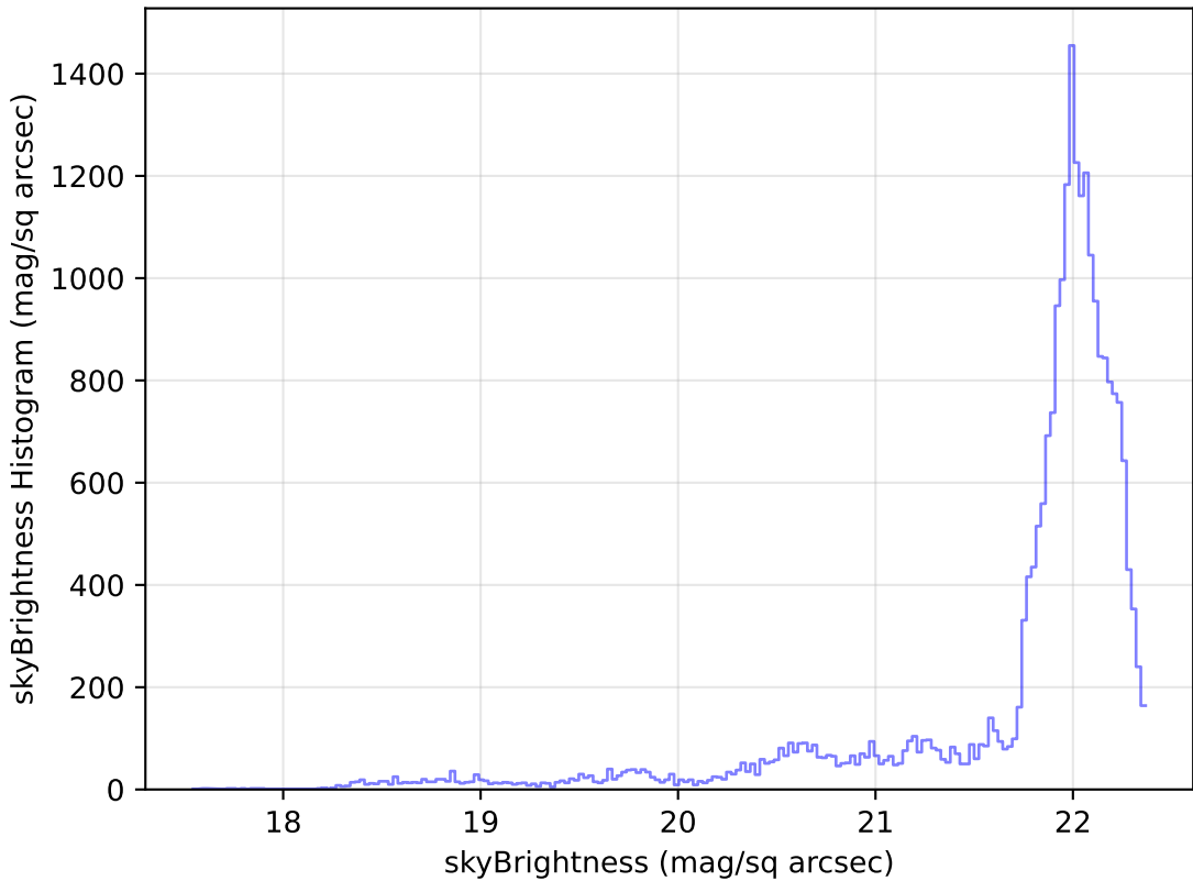
too_ignore_100_4v3.4_10yrs Yr 1 g band: skyBrightness Histogram
