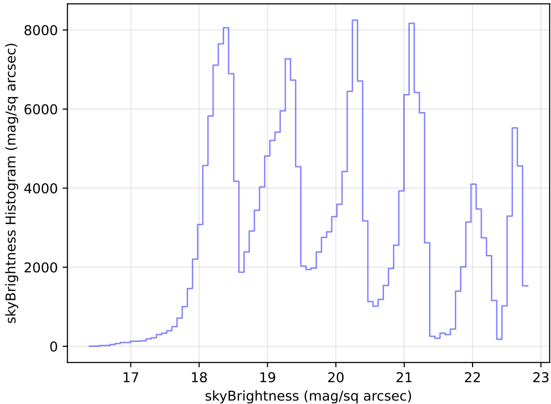
too_ignore_100_4v3.4_10yrs Yr 1 all bands: skyBrightness Histogram
