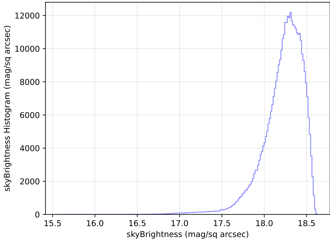
too_ignore_100_4v3.4_10yrs WFD y band: skyBrightness Histogram
