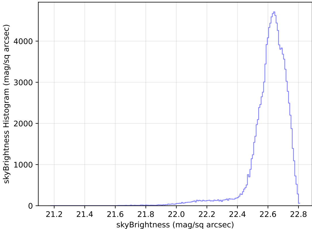
too_ignore_100_4v3.4_10yrs WFD u band: skyBrightness Histogram
