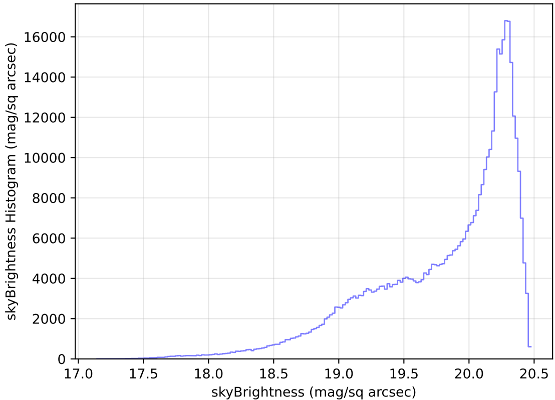
too_ignore_100_4v3.4_10yrs WFD i band: skyBrightness Histogram
