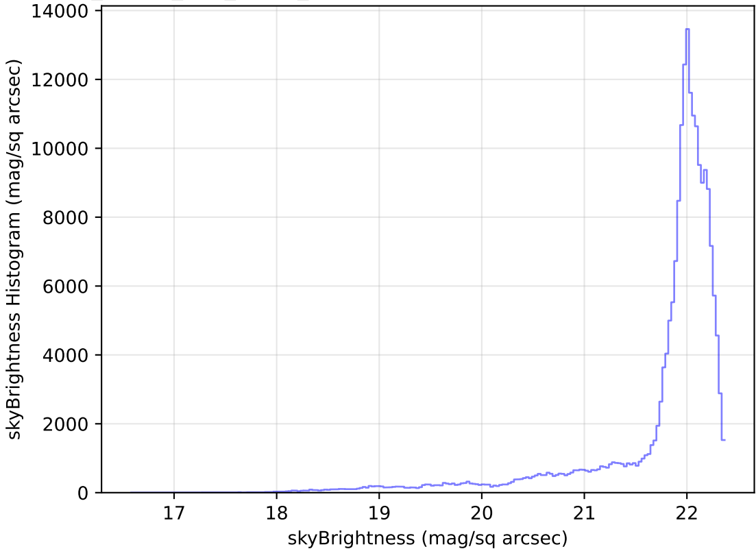
too_ignore_100_4v3.4_10yrs WFD g band: skyBrightness Histogram
