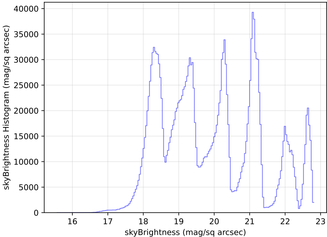
too_ignore_100_4v3.4_10yrs WFD all bands: skyBrightness Histogram
