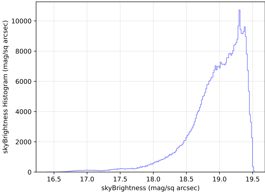
too_ignore_100_4v3.4_10yrs All sky z band: skyBrightness Histogram
