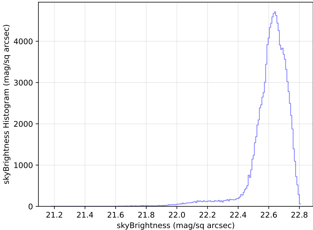
too_ignore_100_4v3.4_10yrs All sky u band: skyBrightness Histogram
