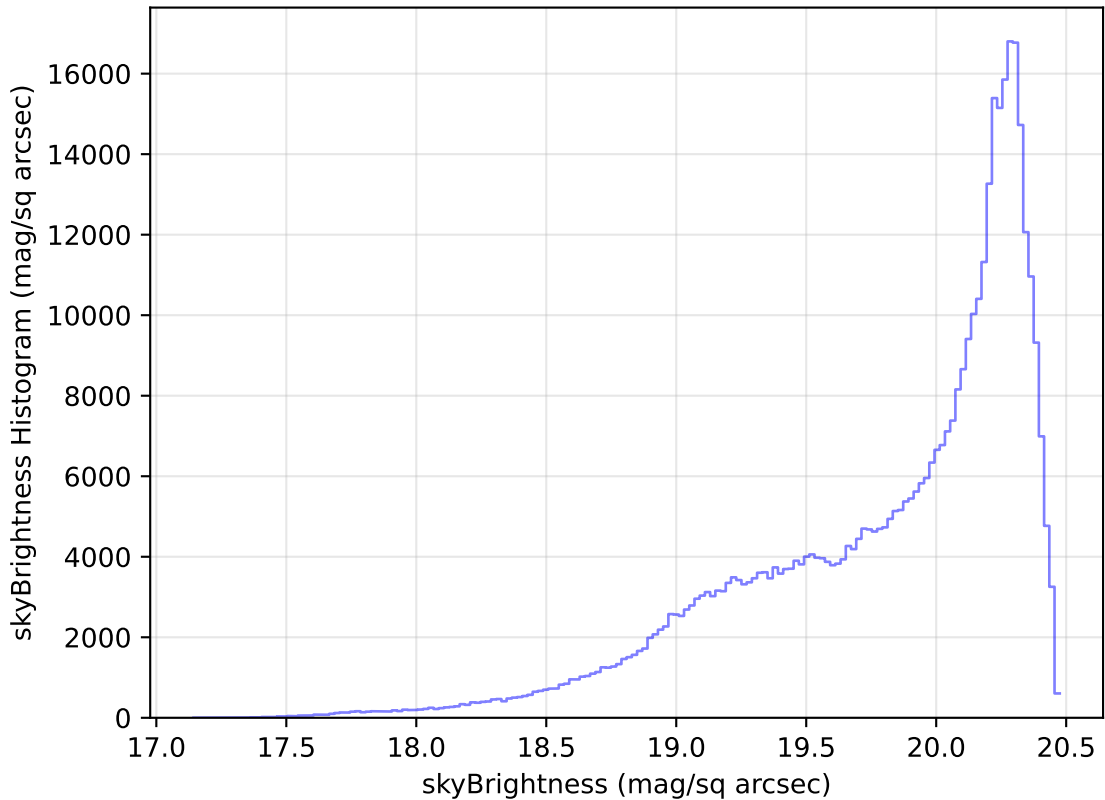
too_ignore_100_4v3.4_10yrs All sky i band: skyBrightness Histogram
