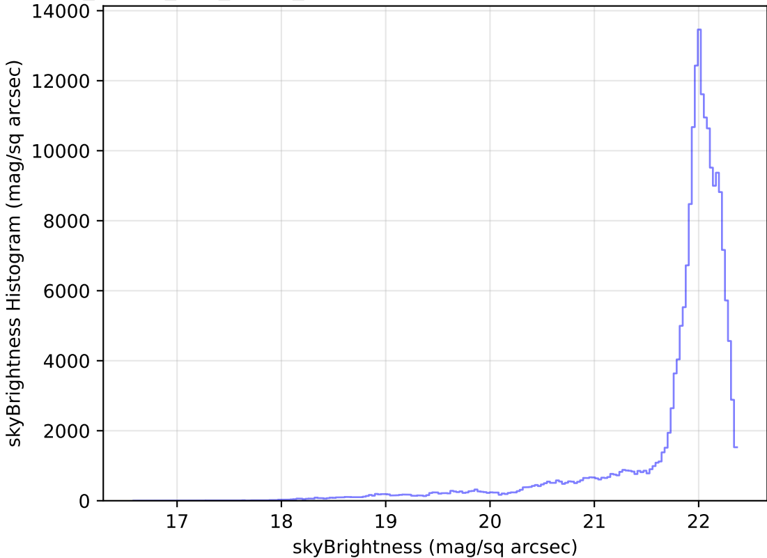
too_ignore_100_4v3.4_10yrs All sky g band: skyBrightness Histogram
