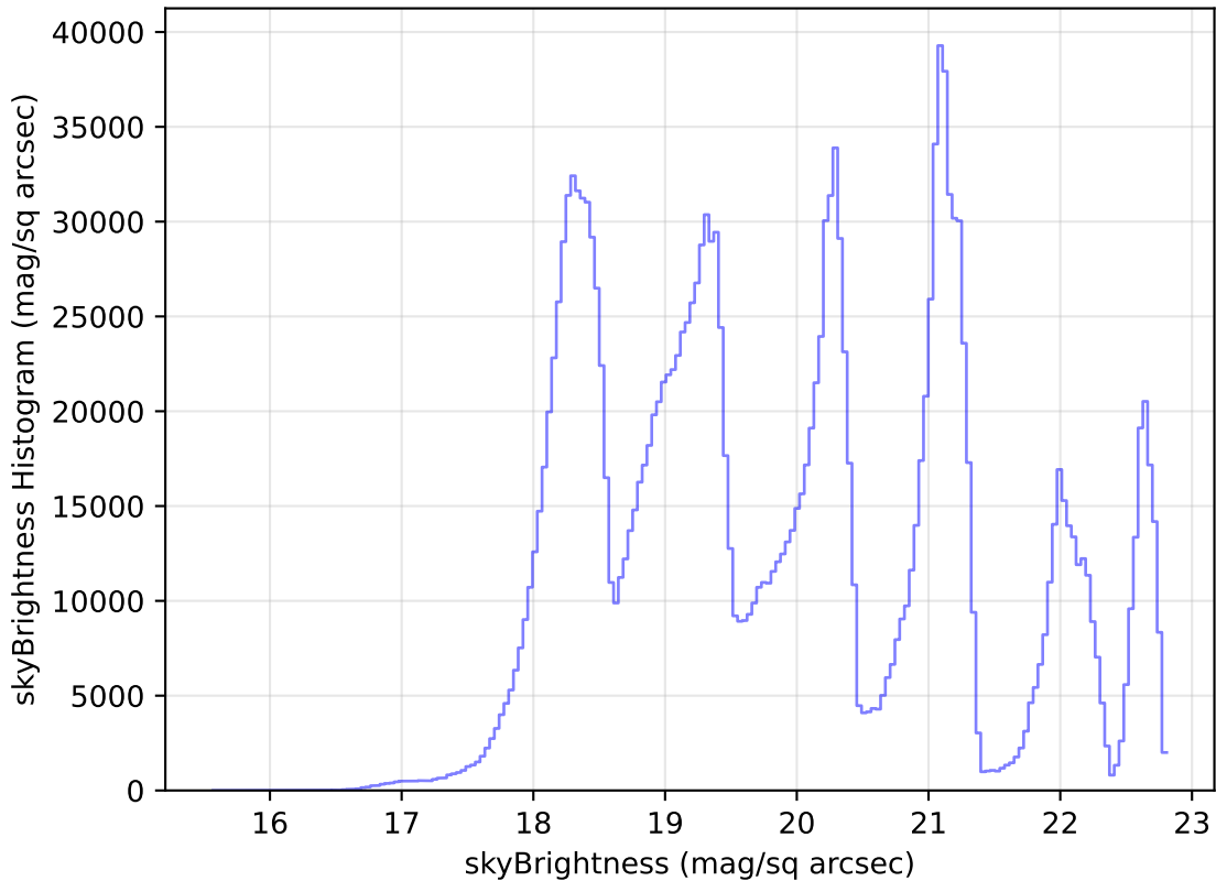
too_ignore_100_4v3.4_10yrs All sky all bands: skyBrightness Histogram
