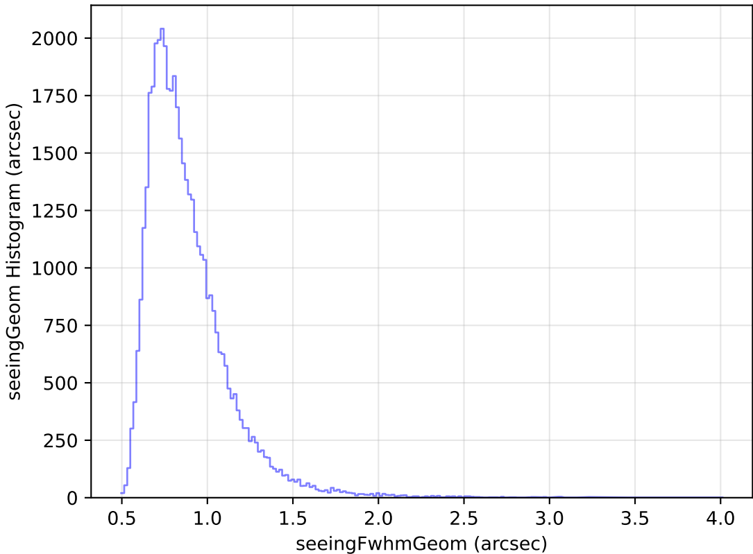
too_ignore_100_4v3.4_10yrs Yr 1 z band: seeingGeom Histogram
