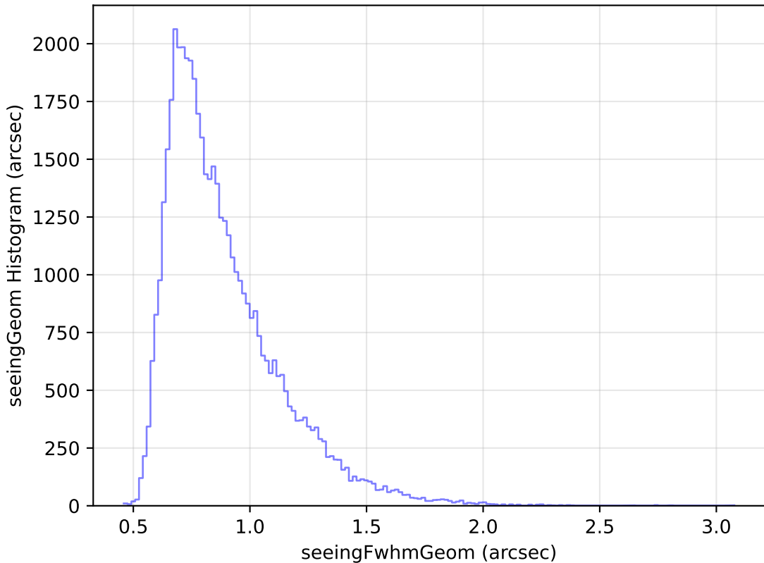
too_ignore_100_4v3.4_10yrs Yr 1 r band: seeingGeom Histogram
