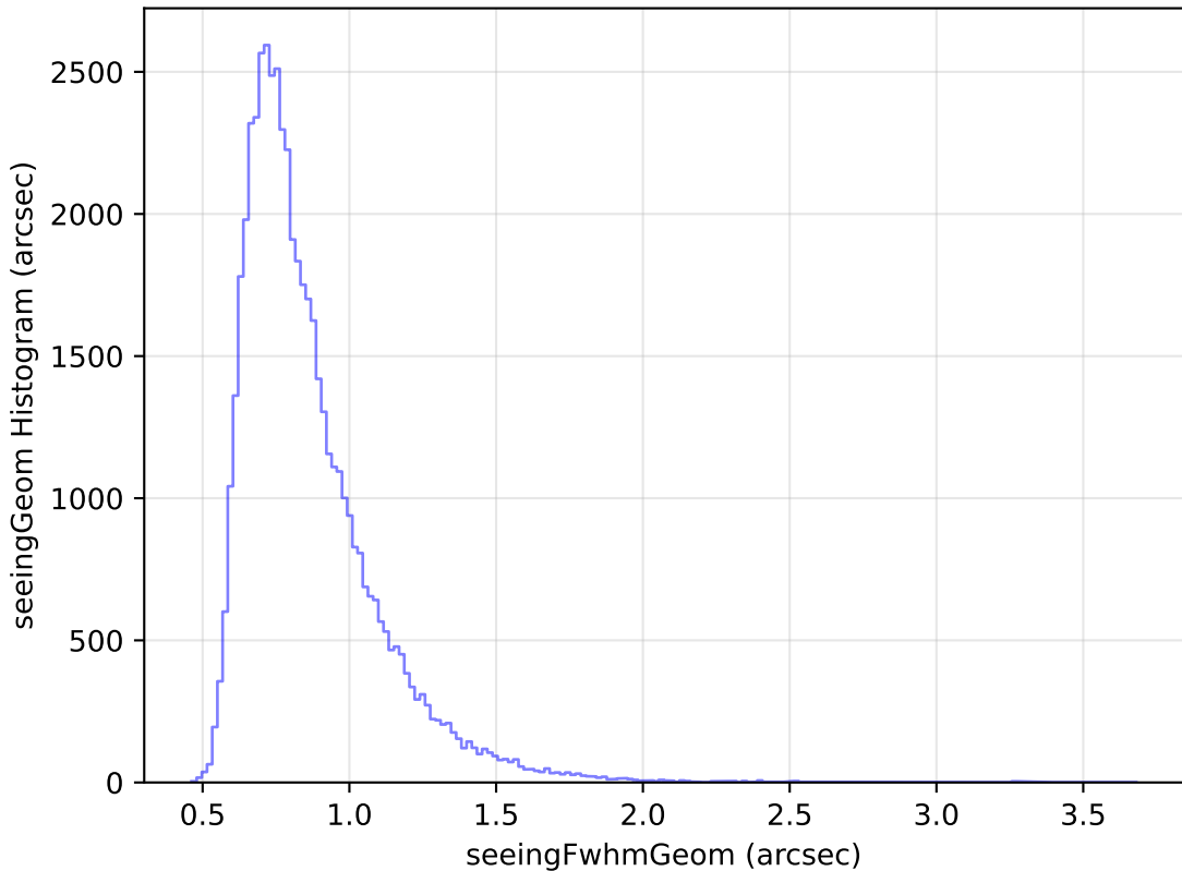
too_ignore_100_4v3.4_10yrs Yr 1 i band: seeingGeom Histogram
