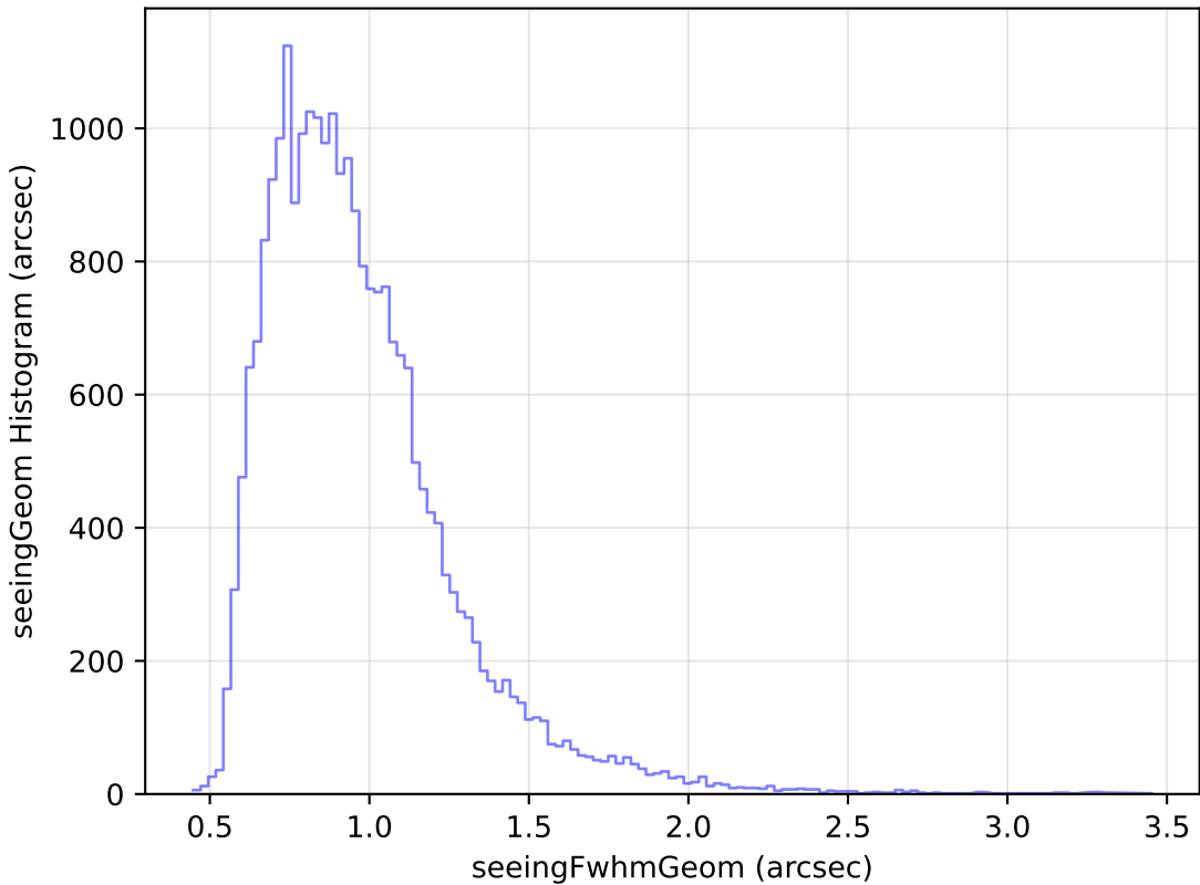
too_ignore_100_4v3.4_10yrs Yr 1 g band: seeingGeom Histogram
