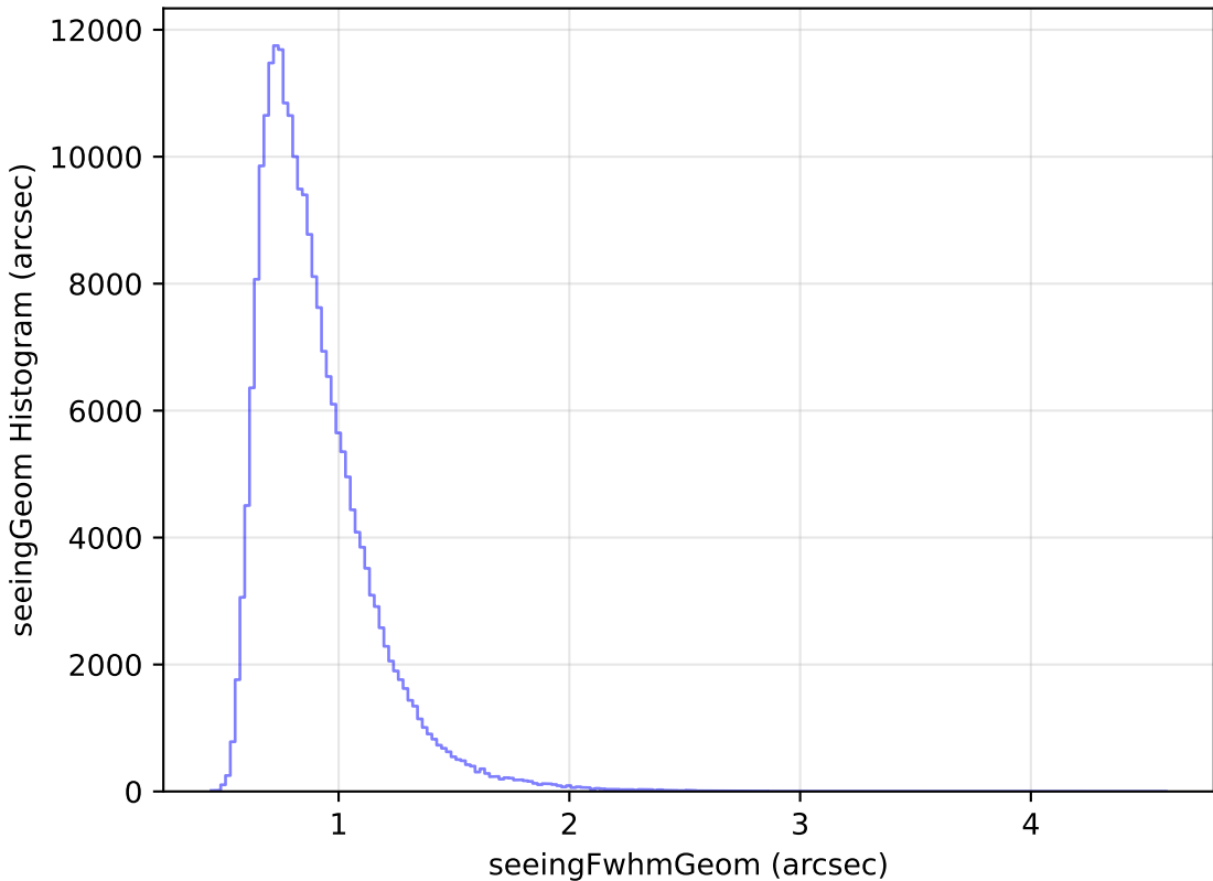
too_ignore_100_4v3.4_10yrs Yr 1 all bands: seeingGeom Histogram
