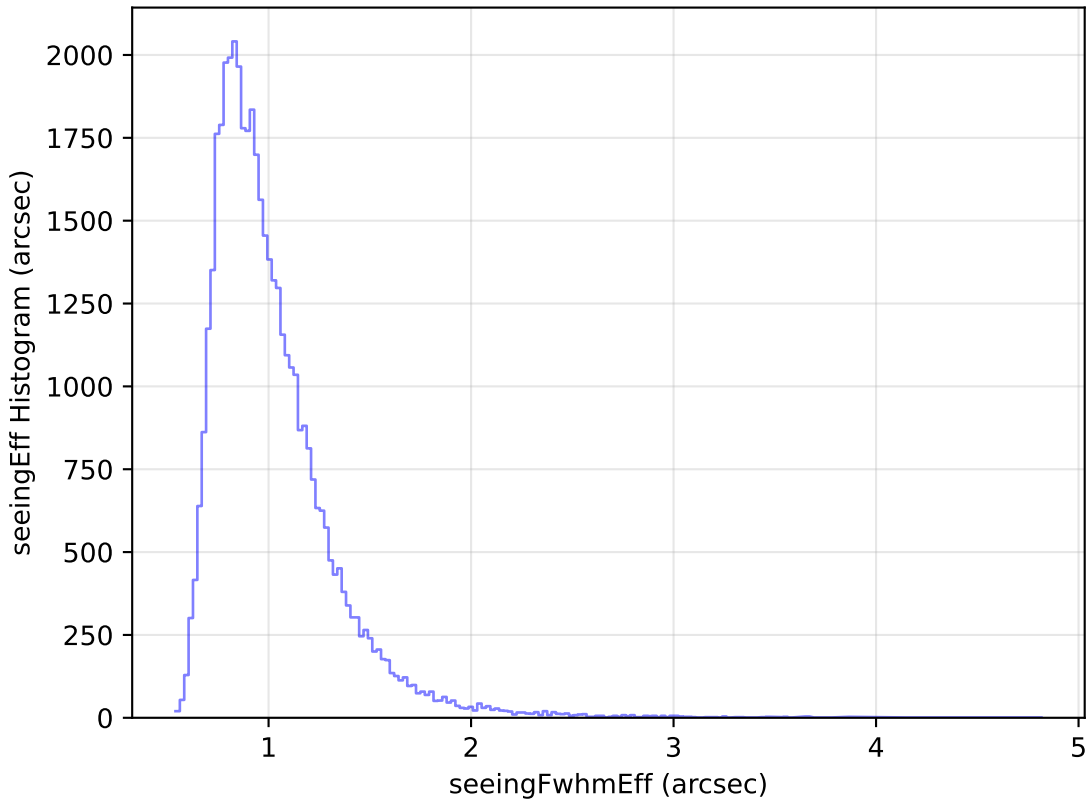
too_ignore_100_4v3.4_10yrs Yr 1 z band: seeingEff Histogram
