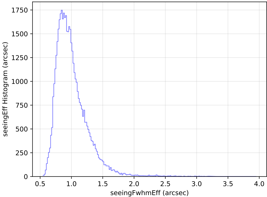
too_ignore_100_4v3.4_10yrs Yr 1 y band: seeingEff Histogram
