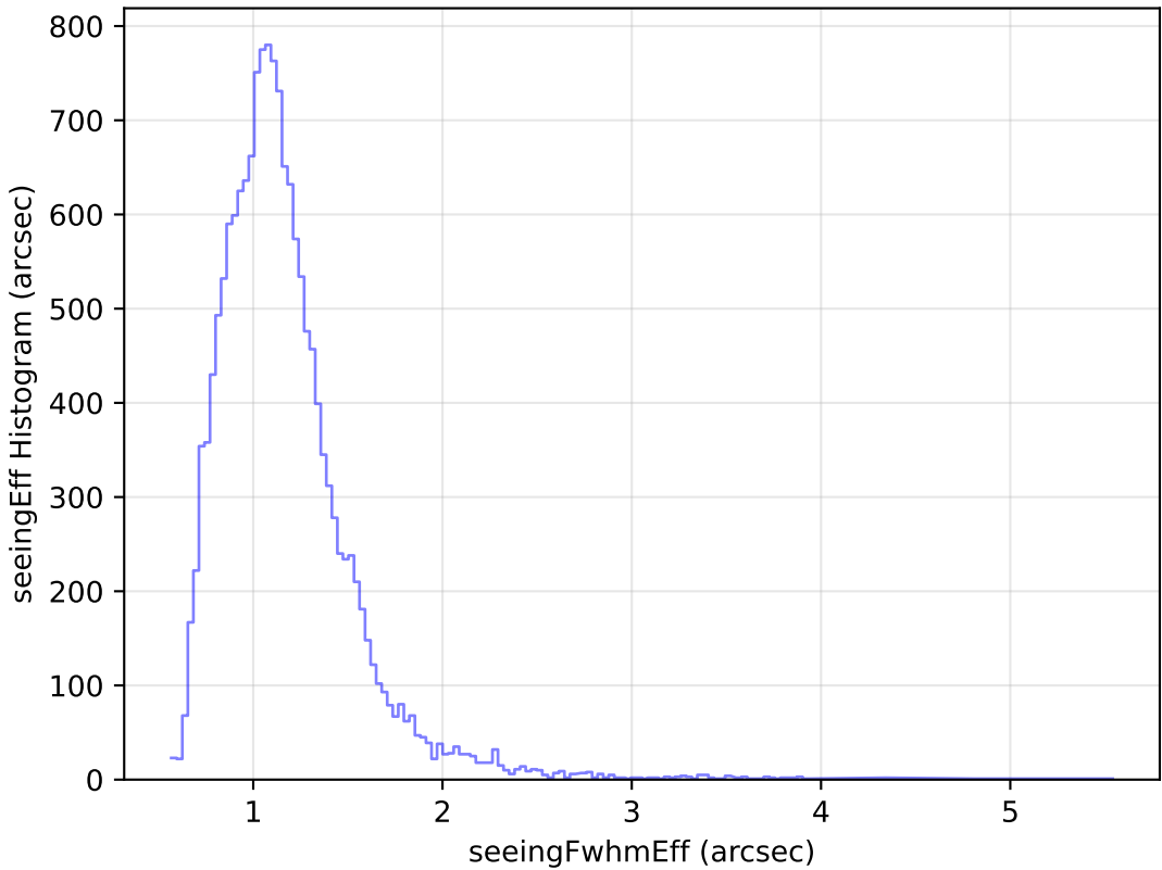
too_ignore_100_4v3.4_10yrs Yr 1 u band: seeingEff Histogram
