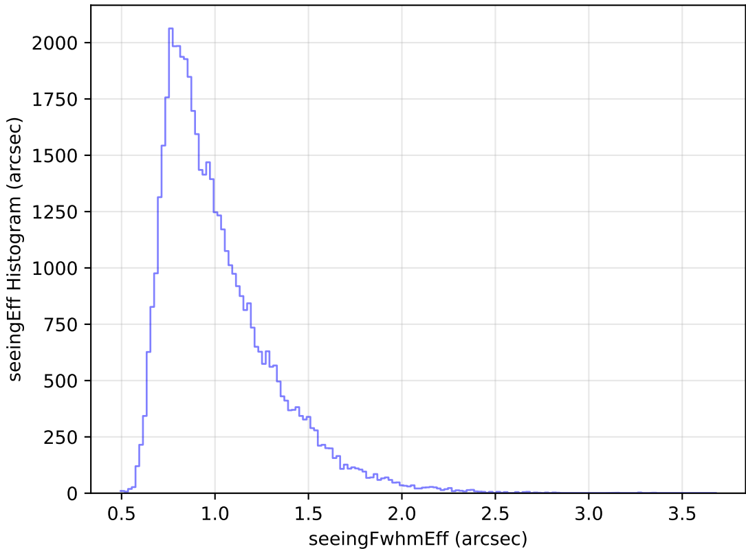
too_ignore_100_4v3.4_10yrs Yr 1 r band: seeingEff Histogram
