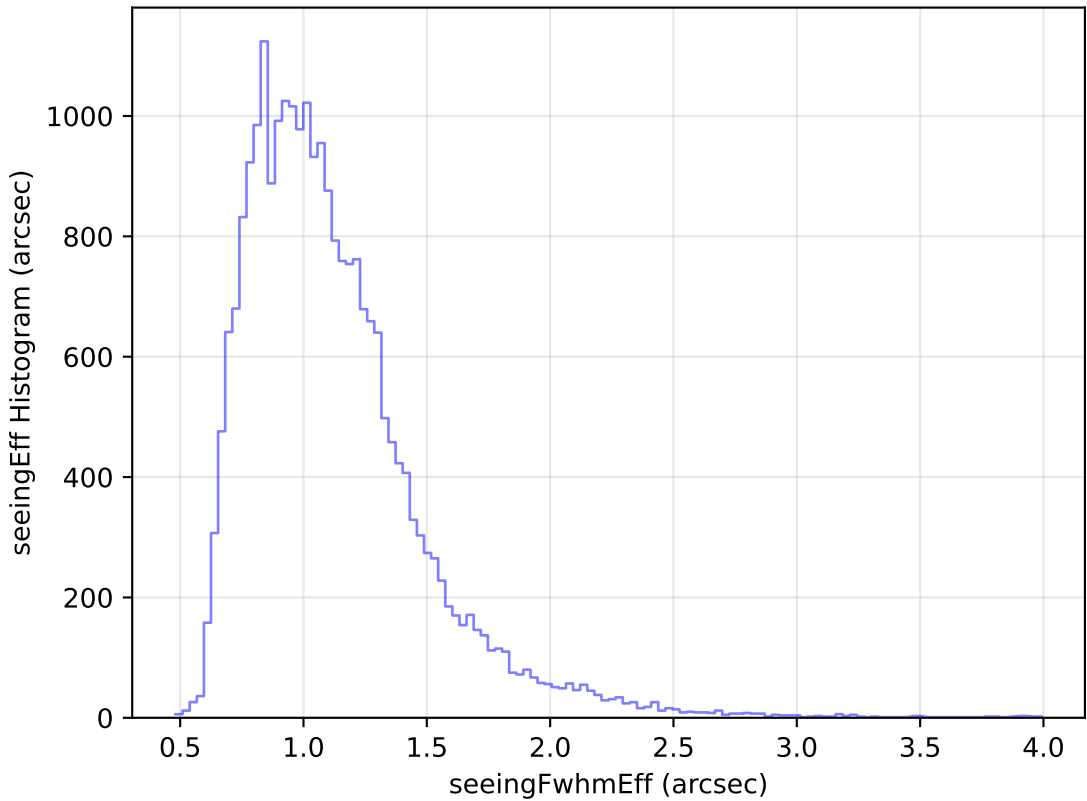
too_ignore_100_4v3.4_10yrs Yr 1 g band: seeingEff Histogram
