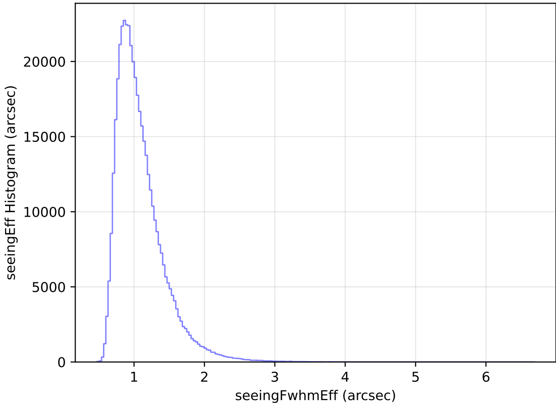
too_ignore_100_4v3.4_10yrs WFD z band: seeingEff Histogram
