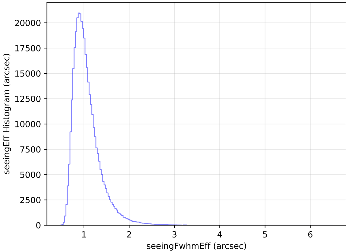
too_ignore_100_4v3.4_10yrs WFD y band: seeingEff Histogram
