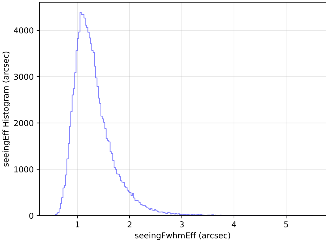
too_ignore_100_4v3.4_10yrs WFD u band: seeingEff Histogram
