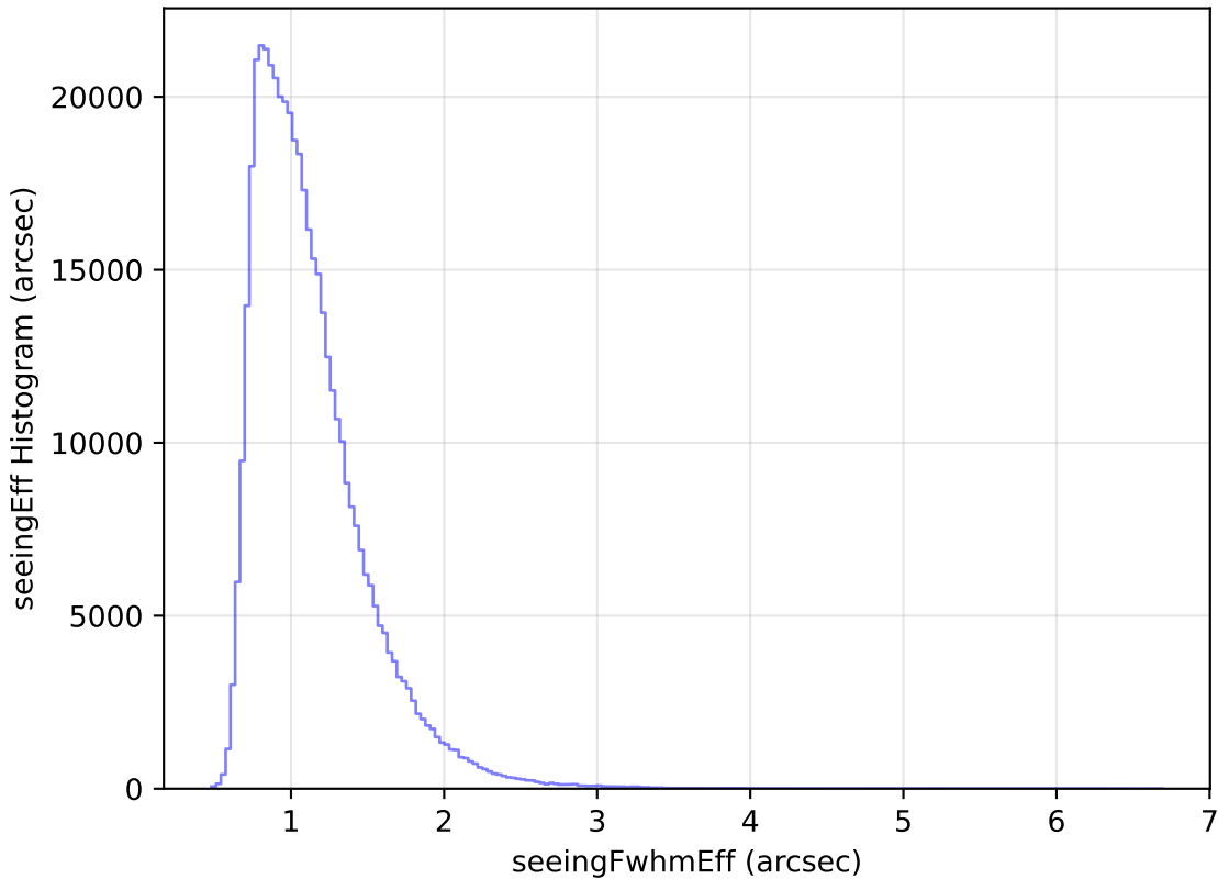
too_ignore_100_4v3.4_10yrs WFD r band: seeingEff Histogram
