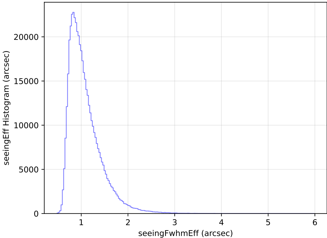
too_ignore_100_4v3.4_10yrs WFD i band: seeingEff Histogram
